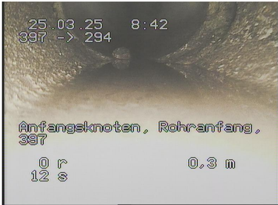
397-294_158.jpg, 00:00:00, 0.00m Anfangsknoten, Rohranfang, 397
