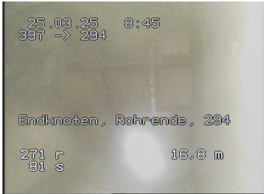
397-294_160.jpg, 00:01:43, 16.80m Endknoten, Rohrende, 294
