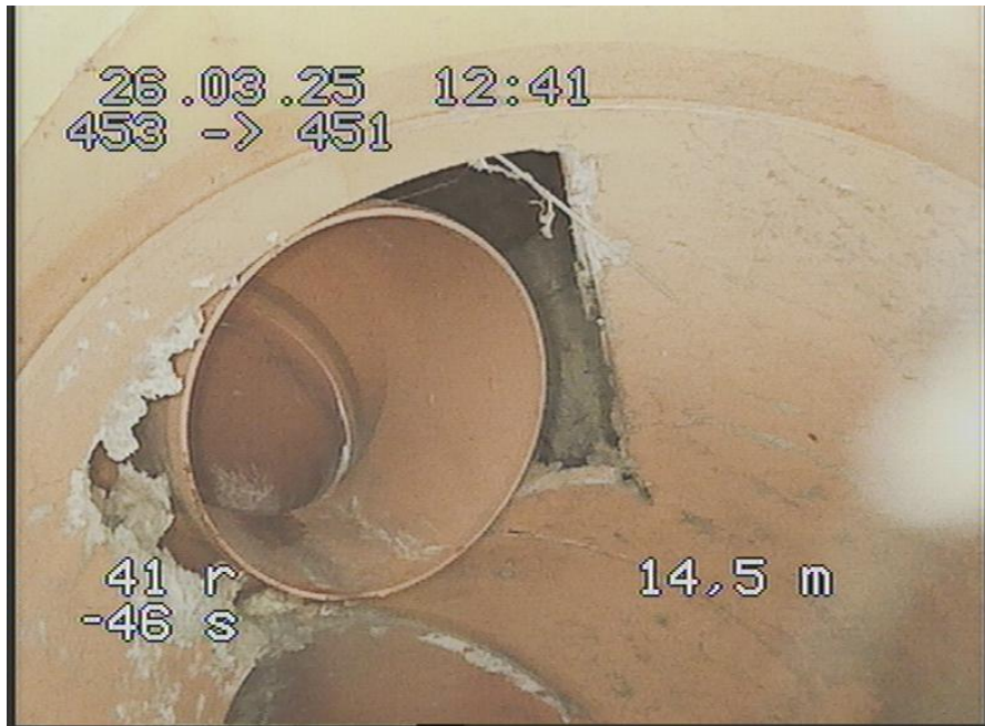
453-451_285.jpg, 00:01:01, 14.50m Endknoten, Rohrende, 453
