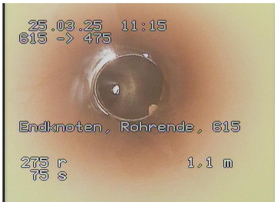
615-475_209.jpg, 00:00:18, 1.10m Endknoten, Rohrende, 615
