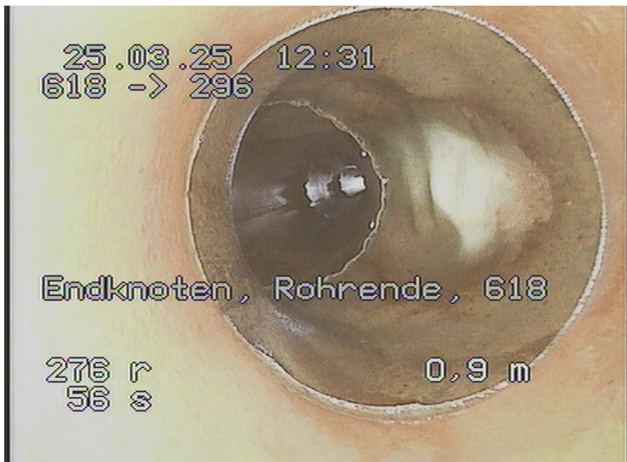
618-296_239.jpg, 00:00:18, 0.90m Endknoten, Rohrende, 618
