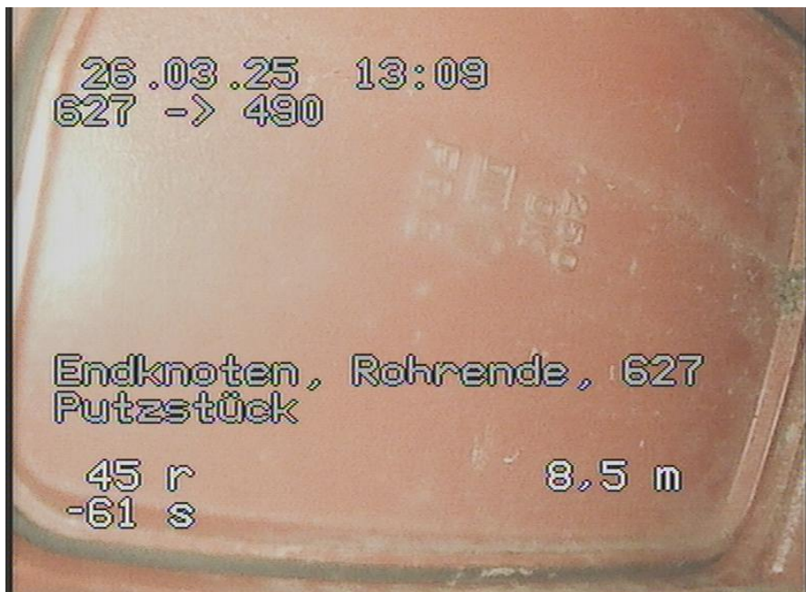
627-490_290.jpg, 00:03:58, 8.50m Endknoten, Rohrende, 627 / Putzstück
