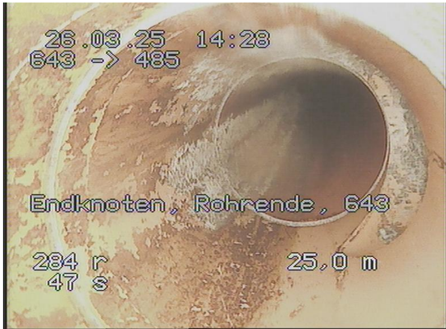
643-485_322.jpg, 00:02:58, 25.00m Endknoten, Rohrende, 643
