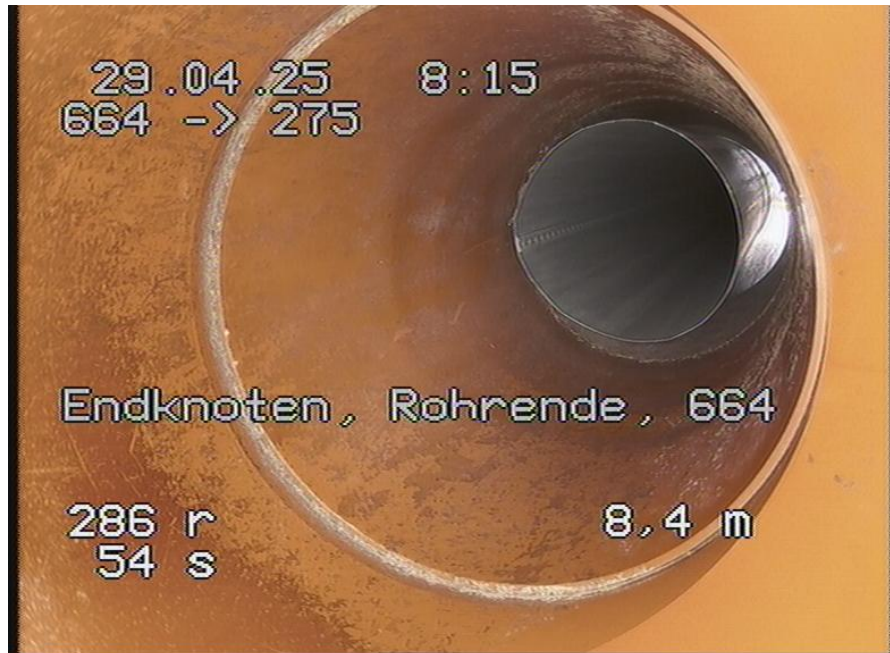
664-275_407.jpg, 00:00:55, 8.40m Endknoten, Rohrende, 664
